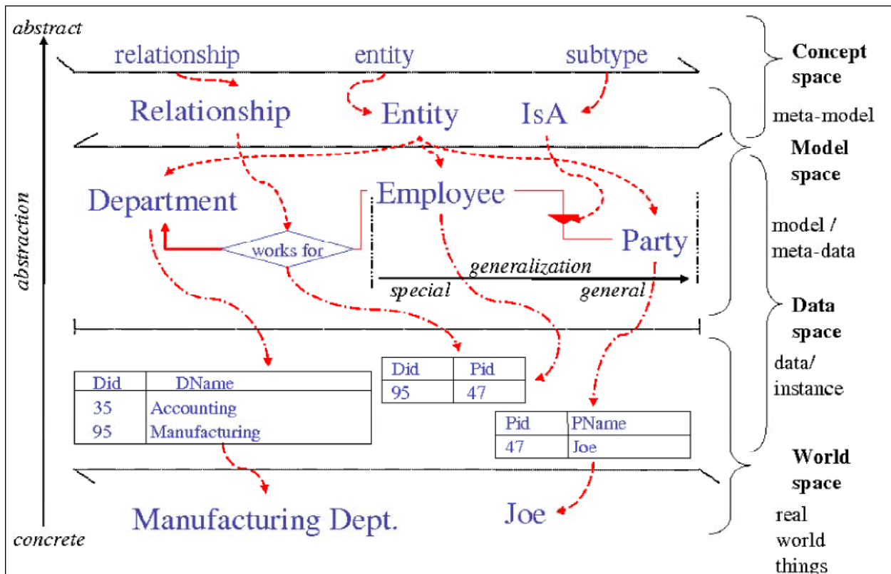
Figure 1. Meta Relationships Example
